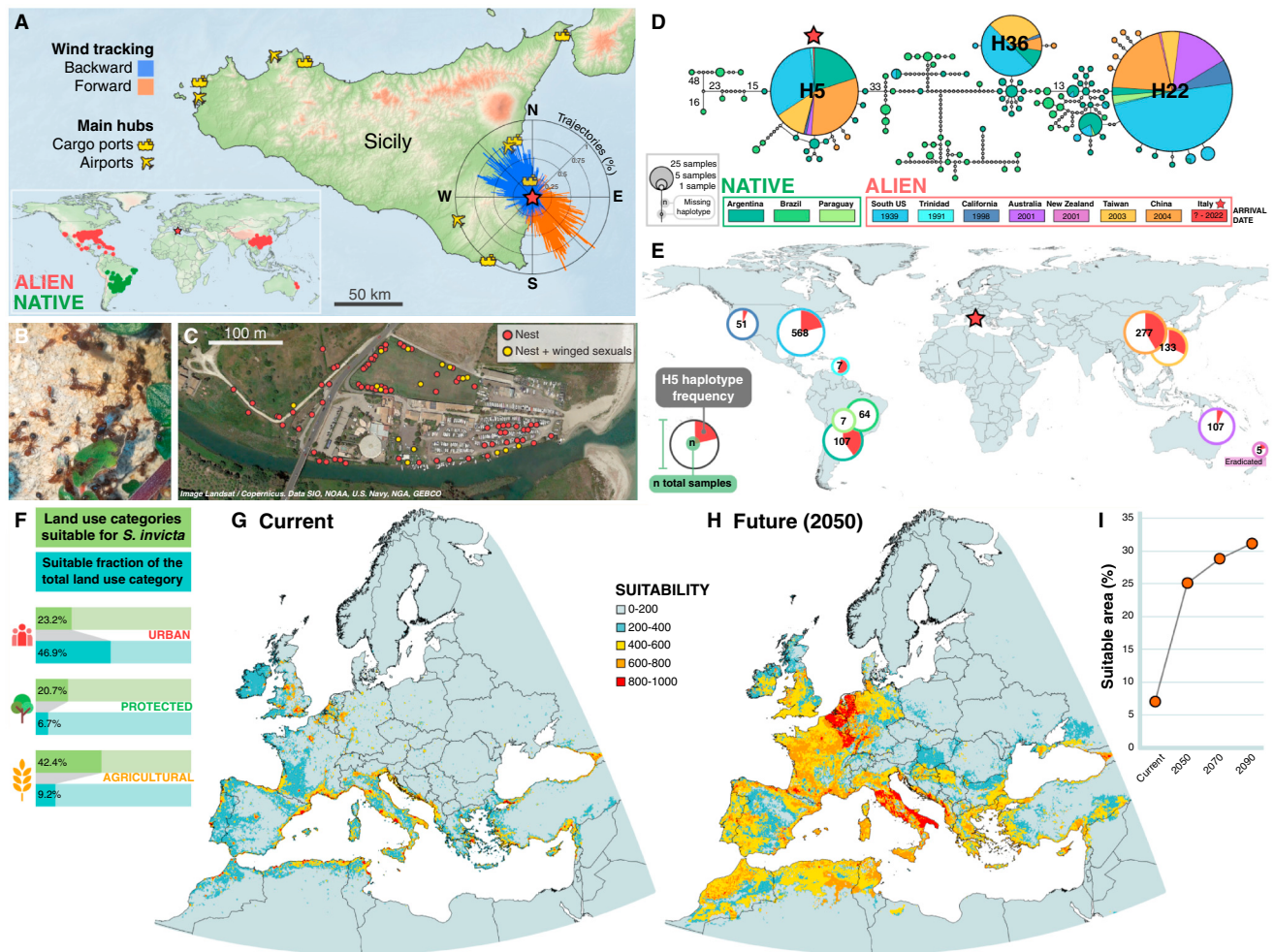
Figure 1. Location, genetic analysis, and modeling of the potential spread of the new alien population of S. invicta .
