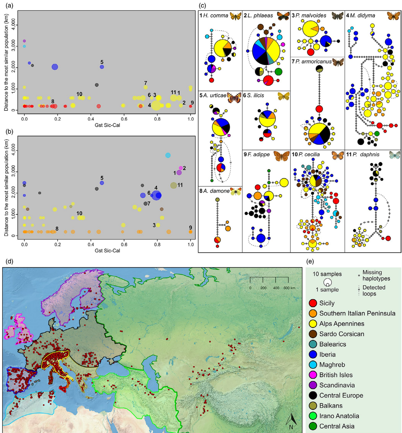
FIGURE 4 The relationships of G st between Sicily and SIP and the ground distance to the genetically closest population from SIP (a) and Sicily (b). The radius of the circles represents the overall p-distance between the populations from Sicily (a) or SIP (b) and the genetically closest populations. The colours of the dots in (a) and (b) indicate the geographic region (d,e) of the genetically closest population. Haplotype networks for 11 species (c), the colours of the sectors indicate the geographic region of specimens described in panels (d) and (e). The numbers in graphs (a) and (b) correspond to the numbers indicated in the haplotype networks in (c). The red dots on the map (d) indicate the sites from which COI sequences were available. [Correction added on 29 June 2020 after first online publication: Caption changed from "... from Sicily (a) and SIP (b)" to "... from SIP (a) and Sicily (b).]
