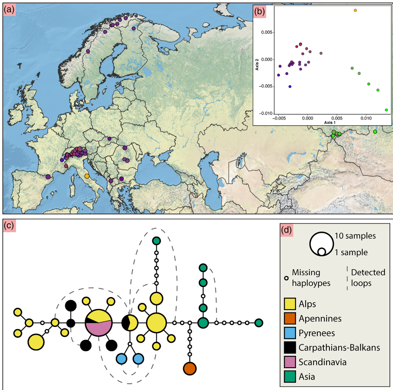
Fig 2. Genetic structure of E. pandrose based on COI sequences: (a) Map of E. pandrose locations (2° resolution) showing where the different COI haplotypes (coloured circles) were collected. Haplotype colours are attributed based on their relative genetic distances by using a PCoA configuration on p-distances projected in RGB space. (b) Relative genetic distance plot among the different E. pandrose haplotypes. Colours association corresponds to Fig. 2a. (c) Maximum parsimony COI haplotype network of E. pandrose . Each line segment represents a mutation between two different haplotypes (coloured circles). According to the legend (d) white dots represent missing haplotypes, dashed lines represent detected loops and circle area is proportional to the number of sequenced specimens possessing a given haplotype. Haplotype colours have been assigned according to the geographic origin of the COI sequences.
